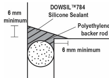
Figure 2: Fillet joint
